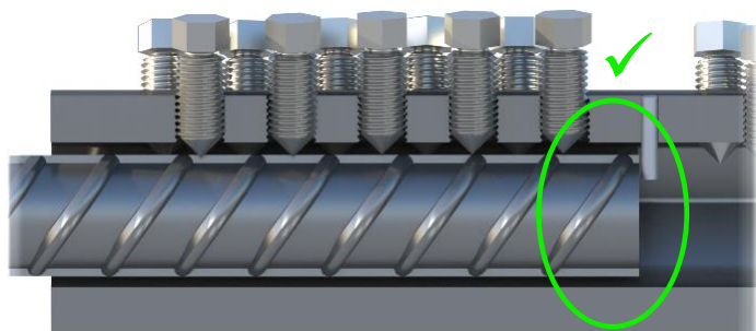
FIGURE 1: Correct Rebar Insertion Depth
