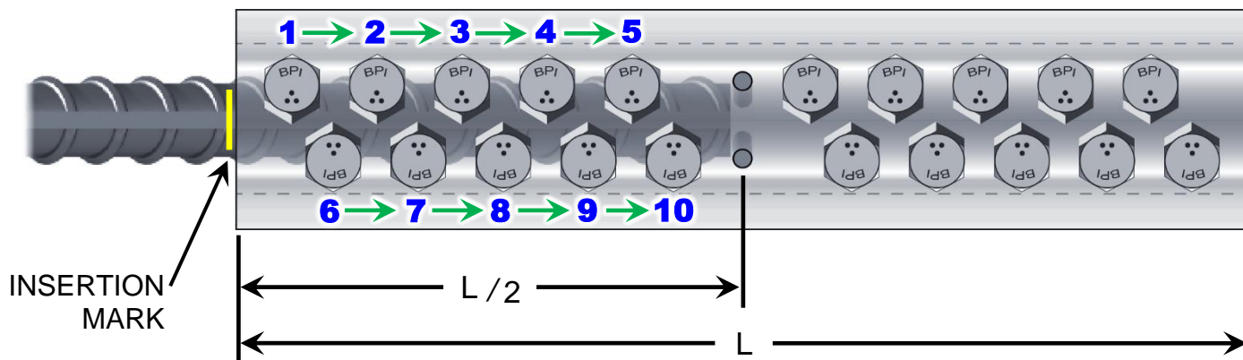
FIGURE 3: Correct Tightening Order, 1 ST Side (#14 shown, #18 similar)
